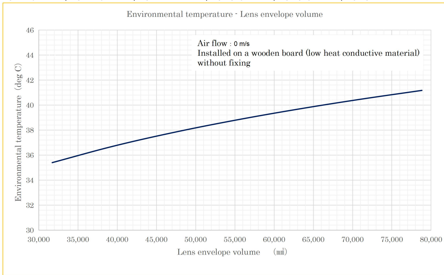
(Reference) Fig1.3-2 Relationship between attached lens size and usable environmental temperature (Camera installation : Worst condition、Device Temp.=70 deg C)
