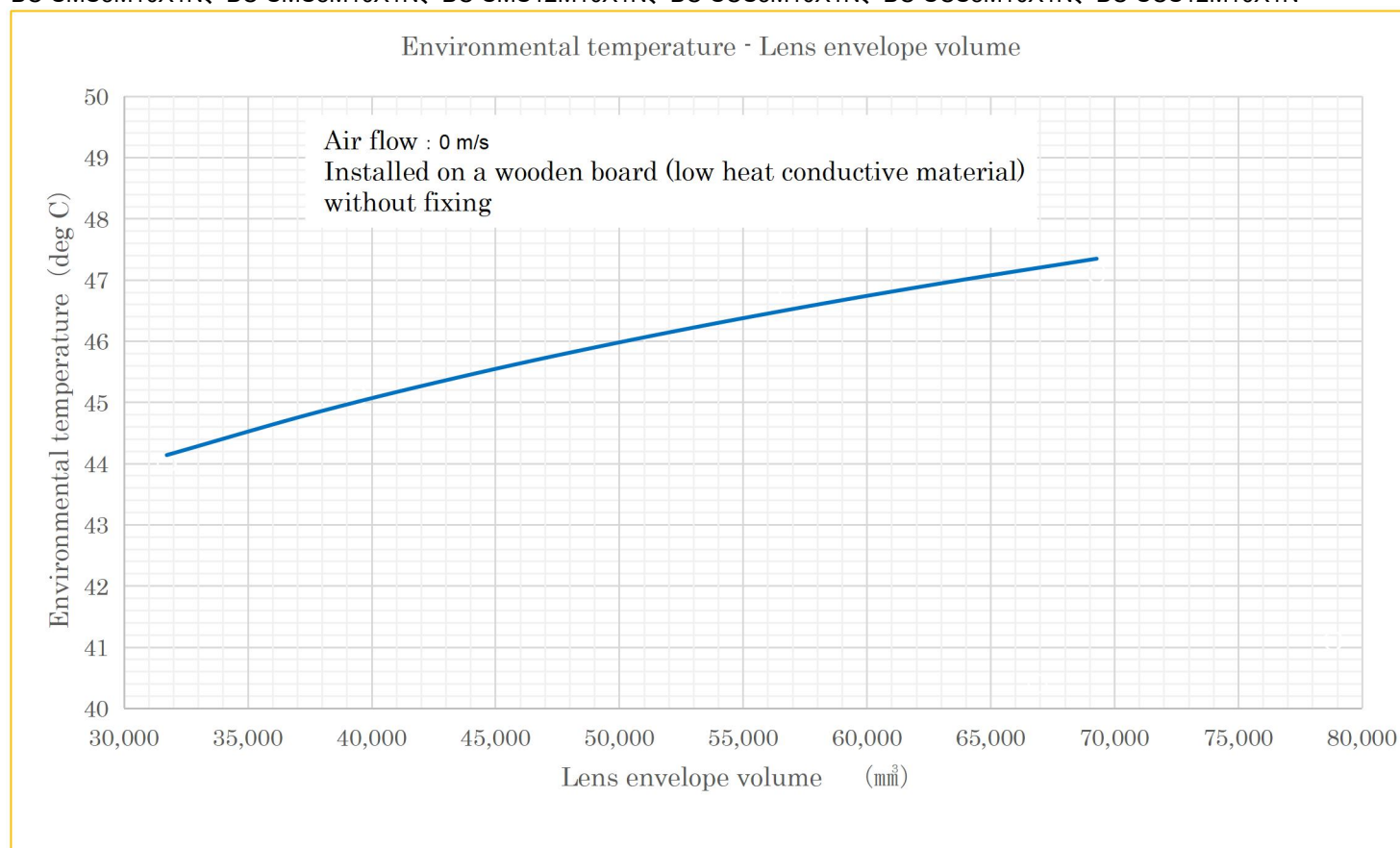
(Reference) Fig1.3-3 Relationship between attached lens size and usable environmental temperature (Camera installation : Worst condition、Device Temp.=70 deg C)
